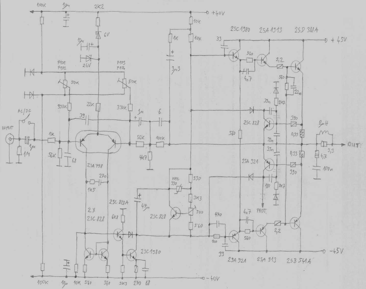
TECHNICS SE-9021 POWER AMP.
