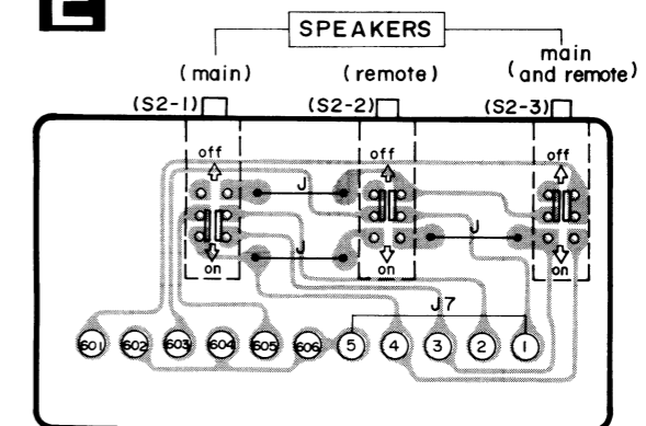
SPEAKER TERMINAL P.C.B.
