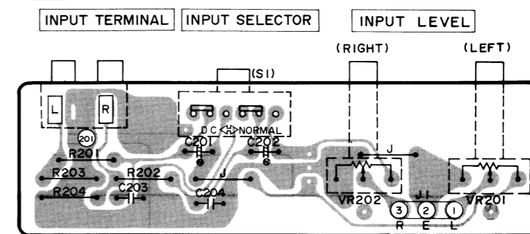
SPEAKERS SELECTOR P.C.B.
