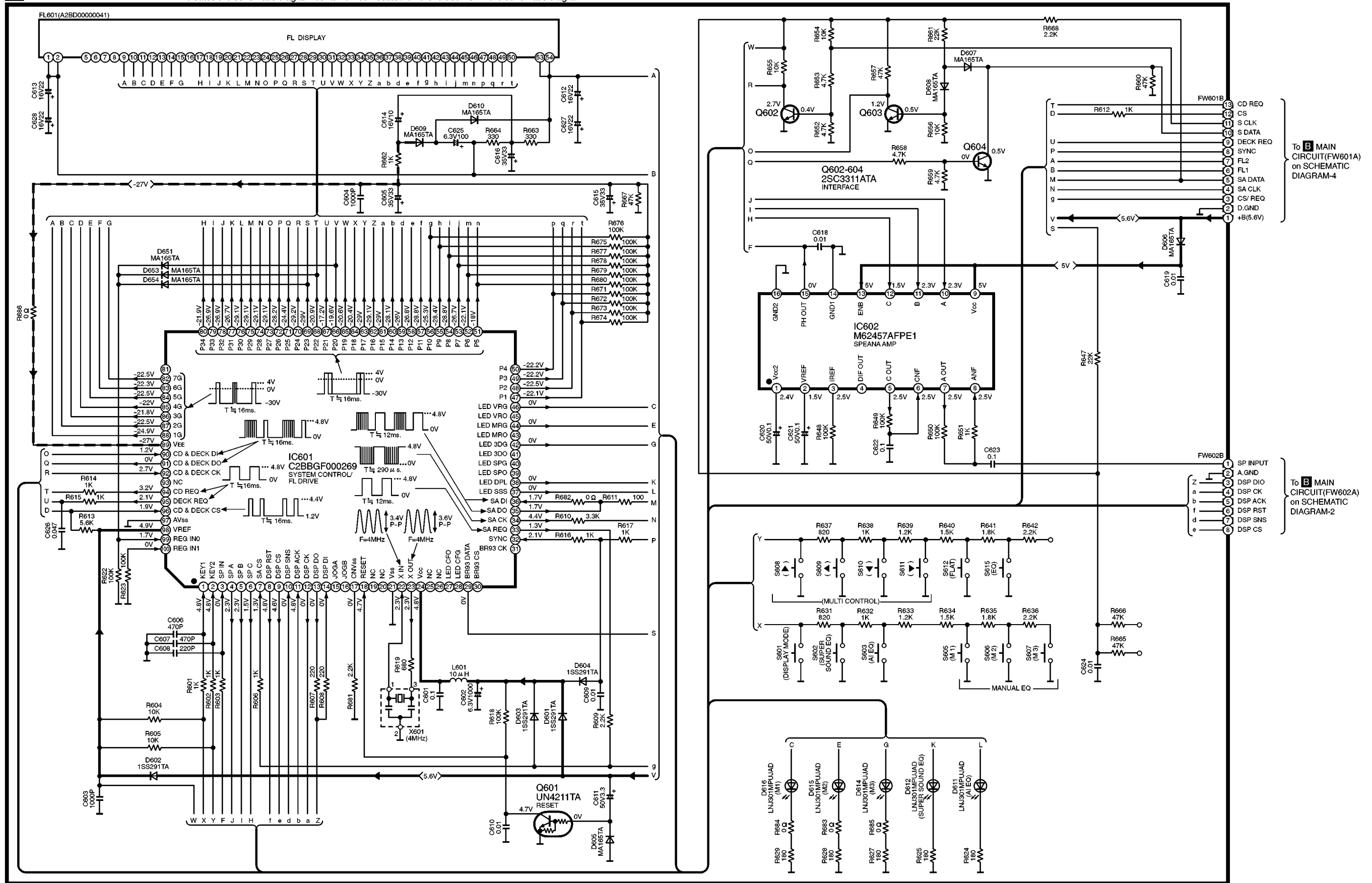
SH-EH580(EG) FL CIRCUIT DIAGRAM
