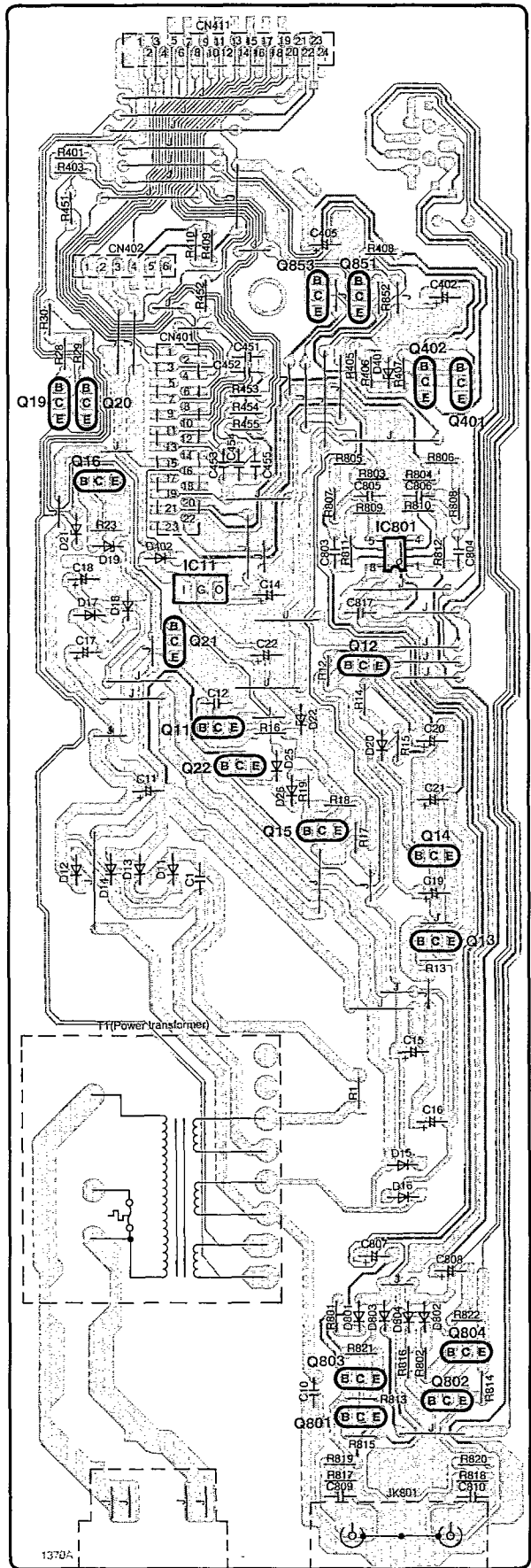
E MAIN P.C.B. (REP2084B-1M)
