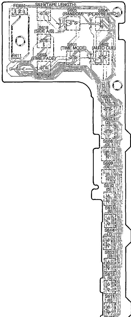
C OPERATION P.C.B. (REP2085A-S)
