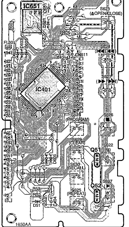
C OPERATION P.C.B. (REP2355A-S)
