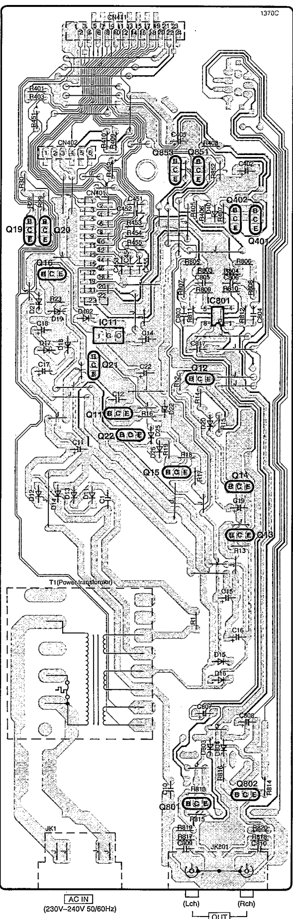
E MAIN P.C.B. (REP2354A-M)
