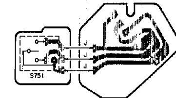
F SWITCH P.C.B. (REP0990)
