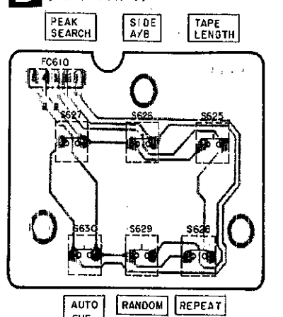
D OPERATION (2) P.C.B. (REP1385A-S)
