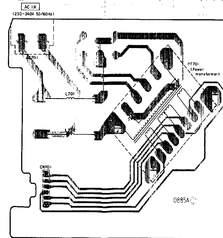
I POWER SUPPLY P.C.B. For (E,EB,EG,GN) areas. (REP1395C-P---(GN) REP1395E-P---(E,EB,EG)
