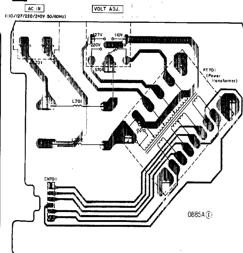
L POWER SUPPLY P.C.B. For (G) area. (REP1395B-P)
