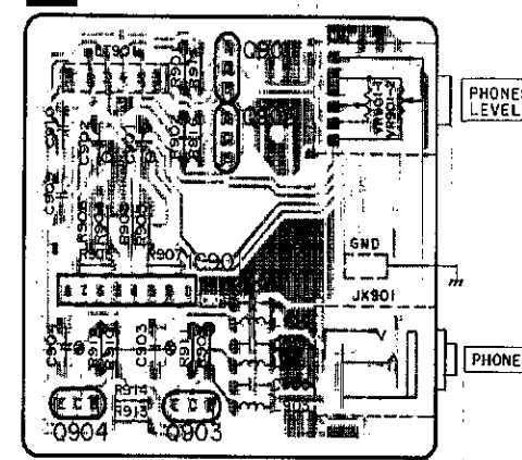
J HEADPHONES JACK P.C.B. (REP1385A-S)
