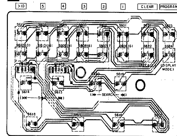
C OPERATION (1) P.C.B. (REP1385A-S)
