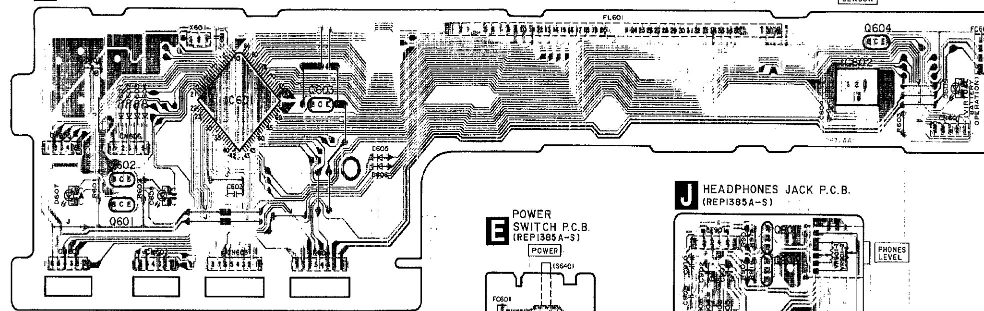
B FL DRIVE P.C.B. (REP1385A-S)
