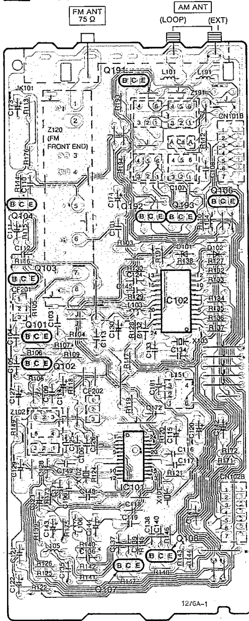
A TUNER P.C.B. (REP1930F-T) For [E] area.
