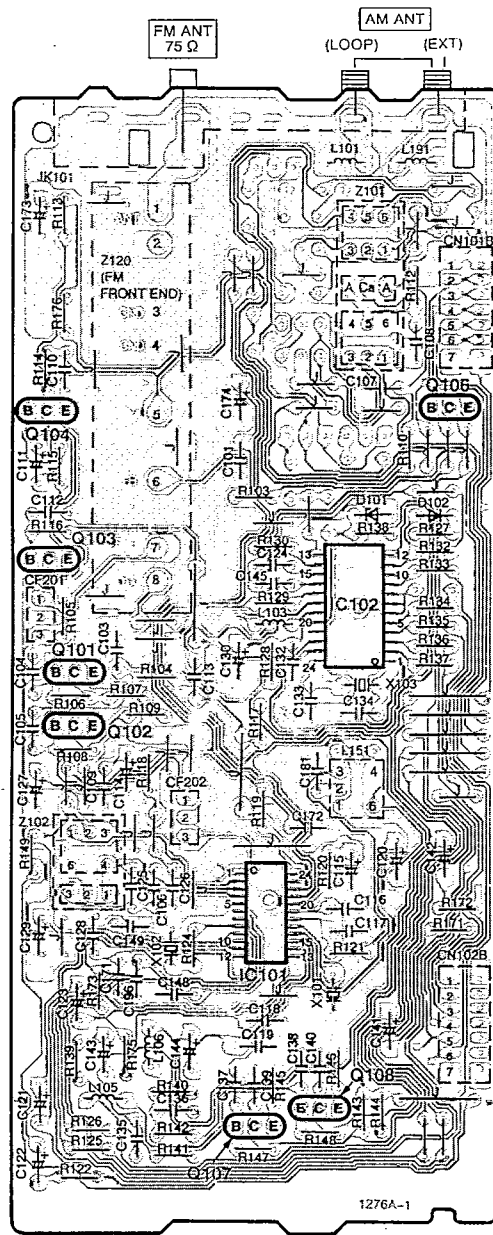
A TUNER P.C.B. (REP1930B-T) For [EG] area.
