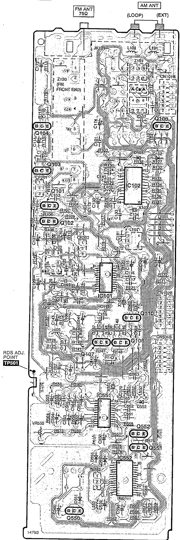
A TUNER P.C.B. (REP2151C-T) For [EG] area.
