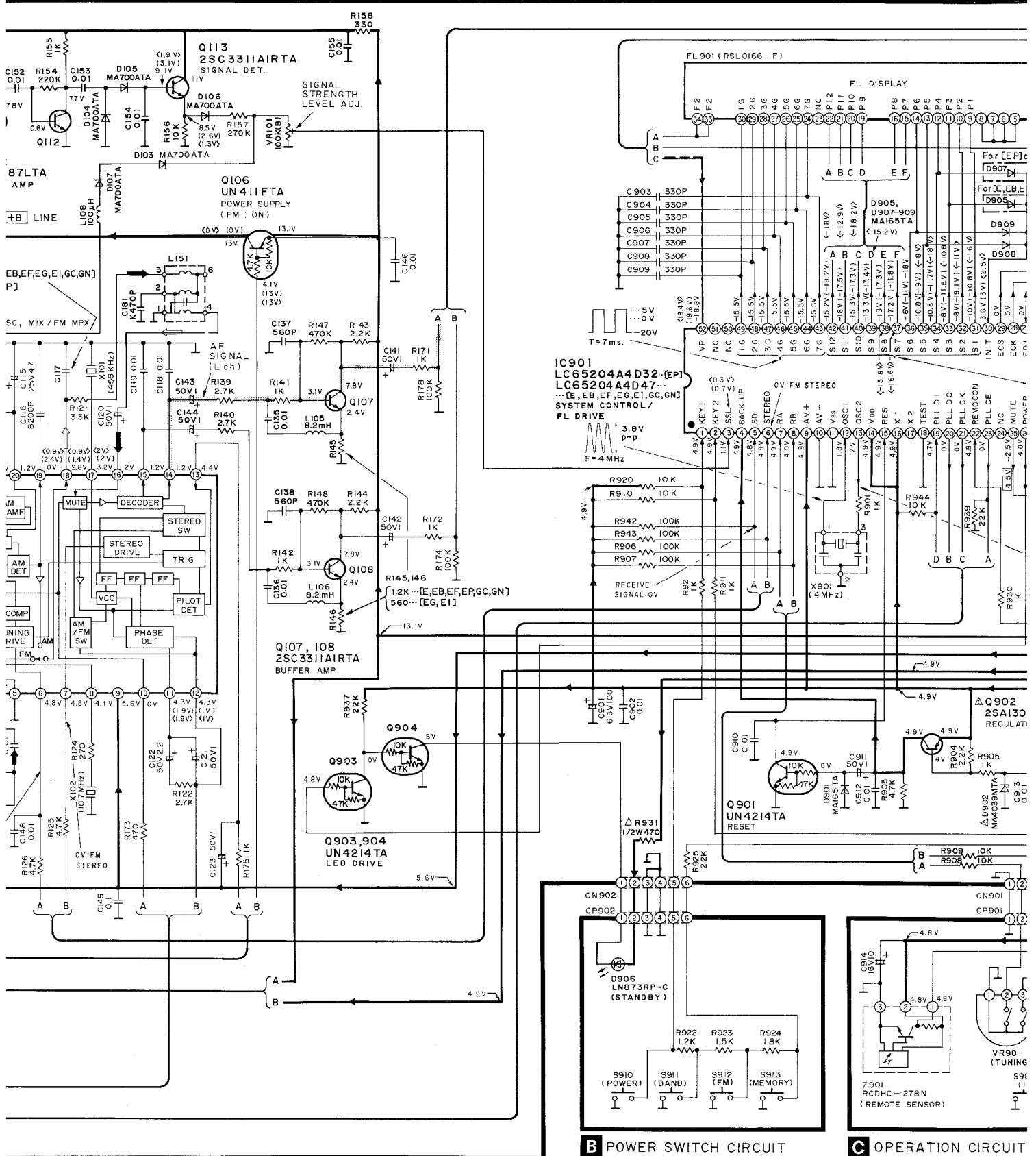
B POWER SWITCH CIRCUIT
