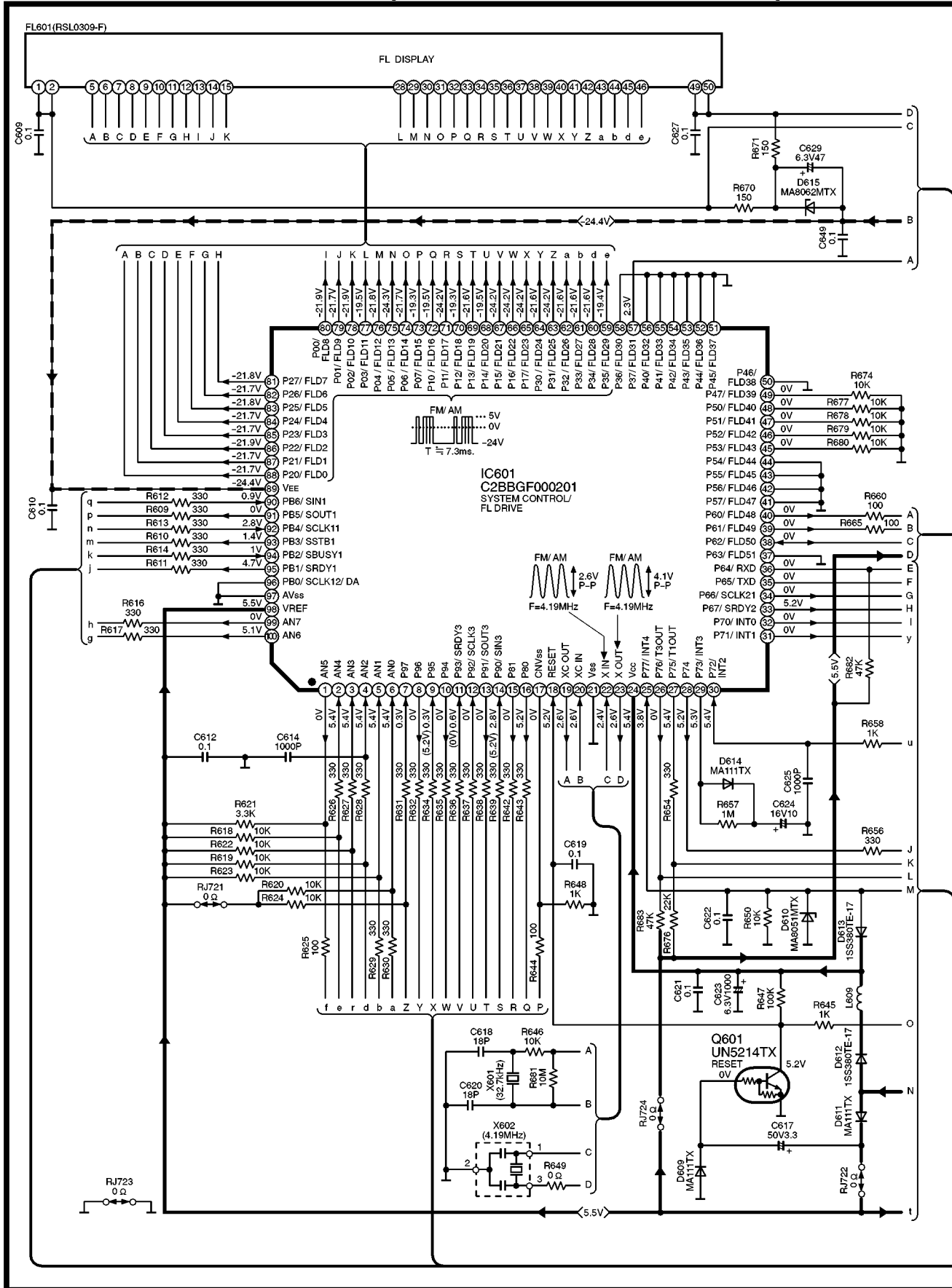
SCHEMATIC DIAGRAM-1
