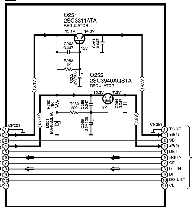
ST-HDA800(E) MAIN , CONNECTOR , EXT IN TERMINAL CIRCUIT DIAGRAM
