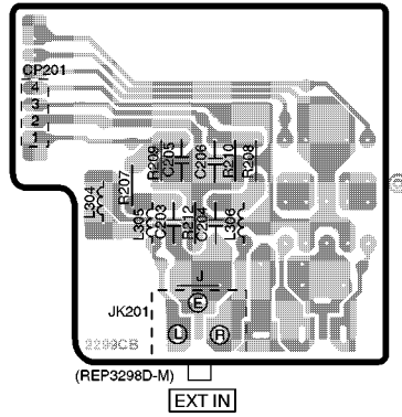
E EXT IN TERMINAL P.C.B.
