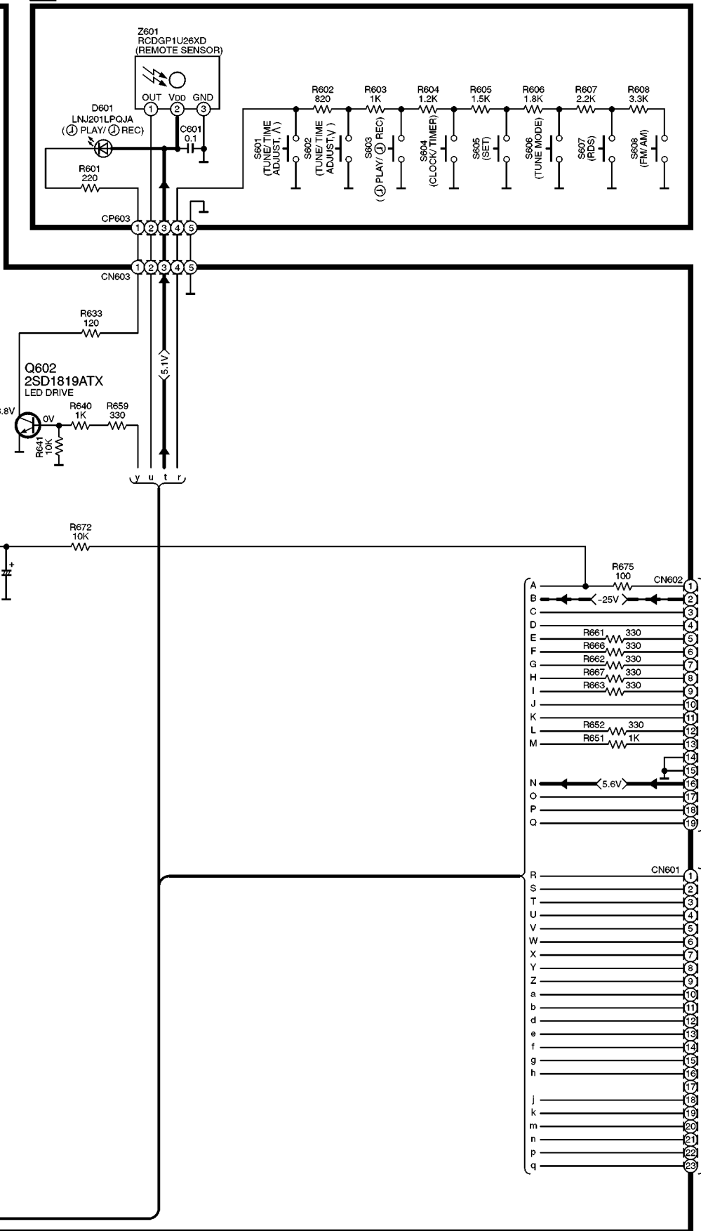
ST-HDA800(E) FL ,OPERATION CIRCUIT DIAGRAM
