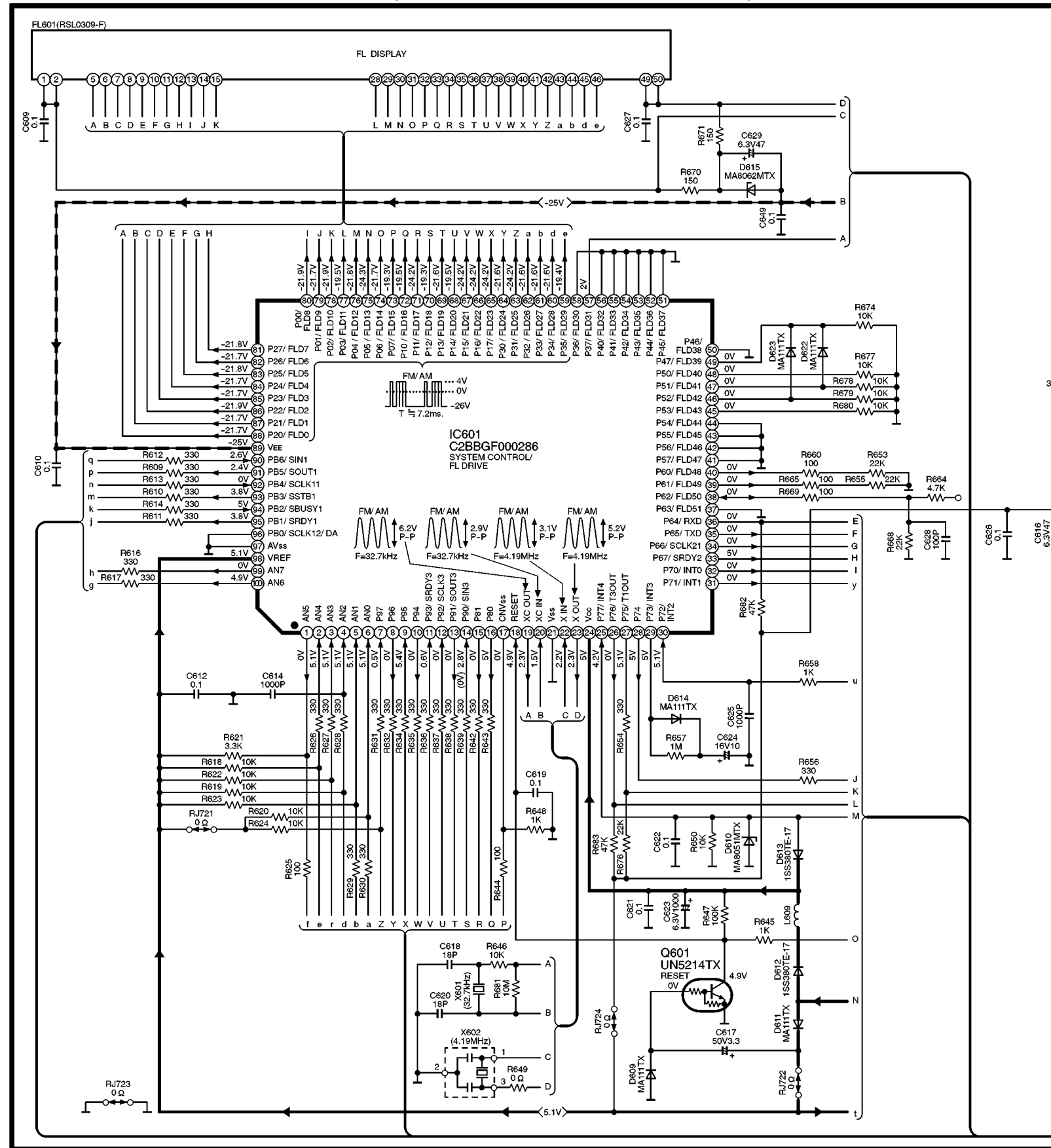
SCHEMATIC DIAGRAM-1
