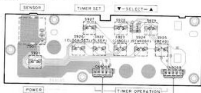
C SENSOR/OPERATION P.C.B.
