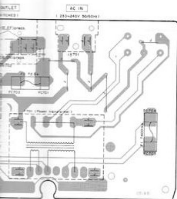
SUPPLY P.C.B. FOR [E,EB,EF,GN] AREAS.
