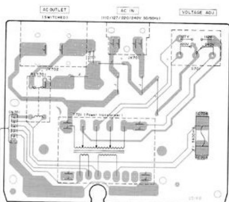
E POWER SUPPLY P.C.B. FOR [GC] AREA.
