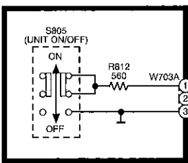
G POWER SWITCH CIRCUIT
