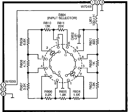
H SELECTOR CIRCUIT
