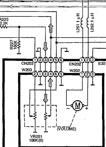
C VOLUME CIRCUIT (P.C. Board: on page 10)
