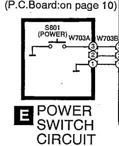
E POWER SWITCH CIRCUIT (P.C. Board: on page 10)
