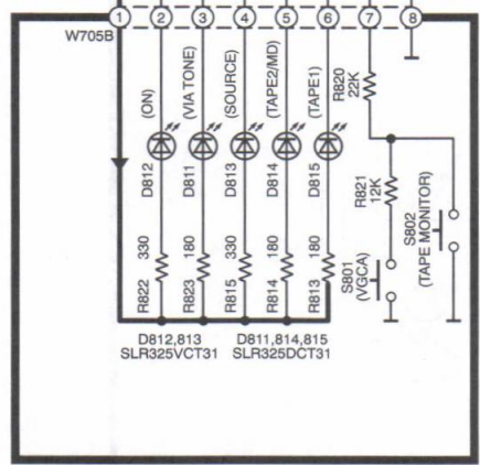
E OPERATION CIRCUIT
