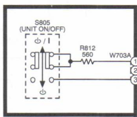
F POWER SWITCH CIRCUIT
