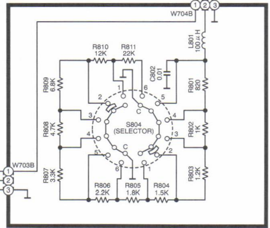
G SELECTOR CIRCUIT
