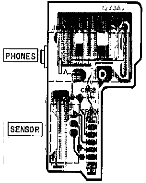
D HEADPHONES JACK P.C.B. (REP1874A-S)
