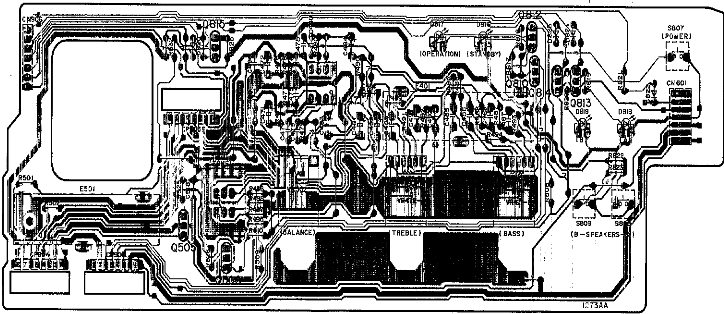
C TONE AMP P.C.B. (REP1874A-S)
