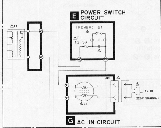
Power Source For [EG] area
