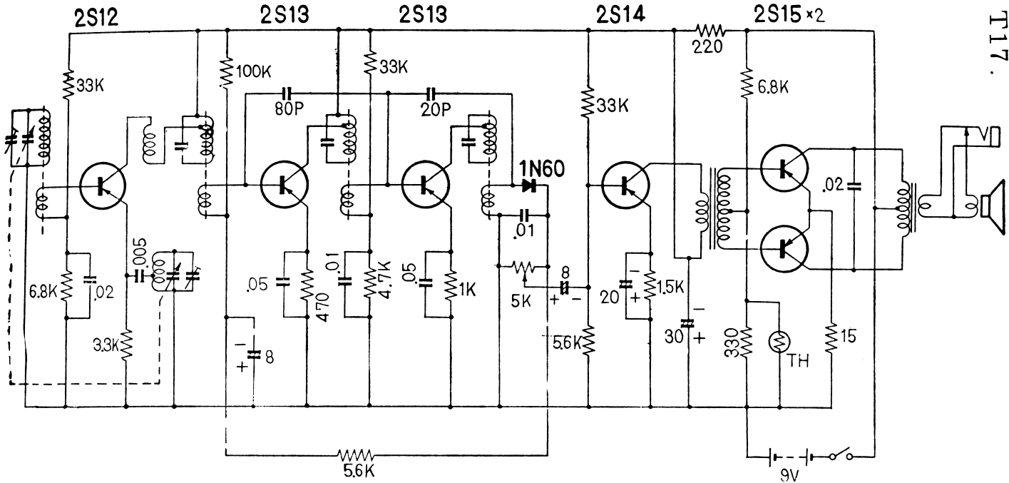
TOSHIBA 6TP-219.
