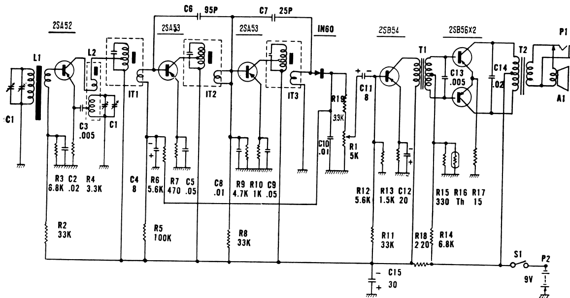
Circuit diagram of "6TP-309"
