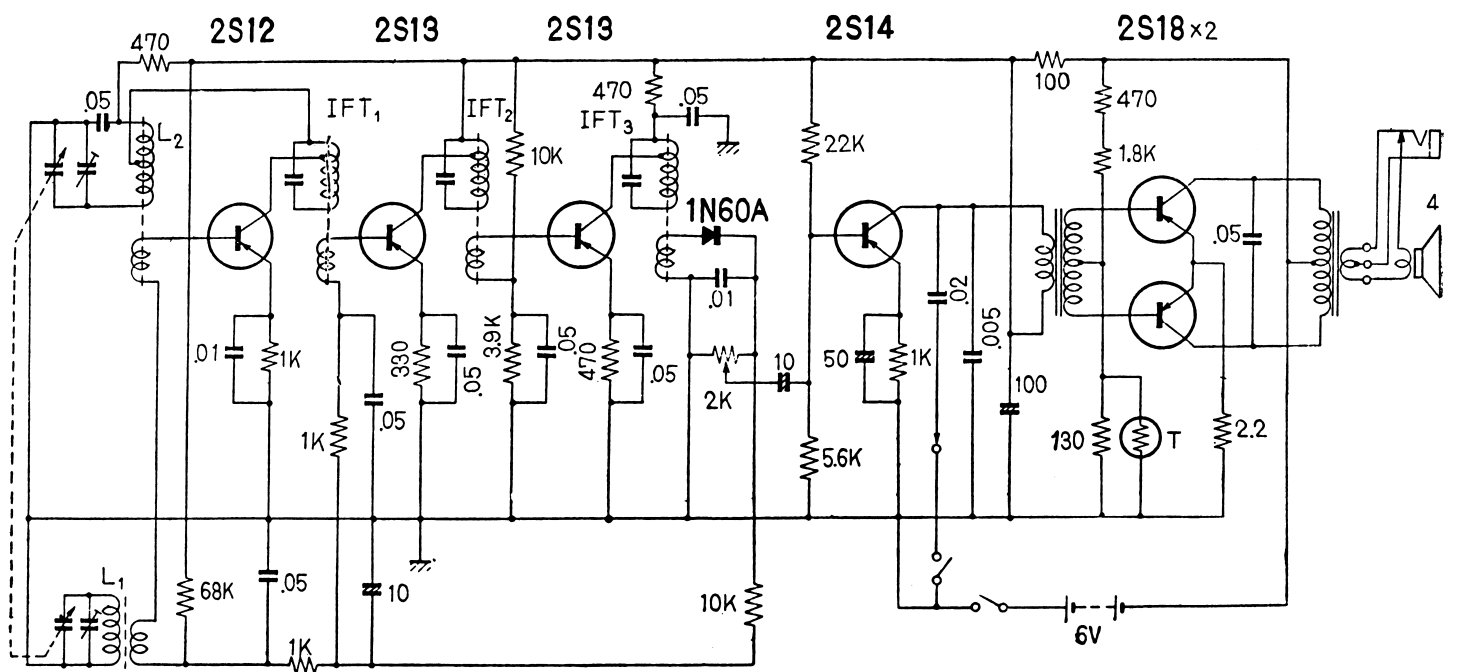
TOSHIBA 6TR-92.
