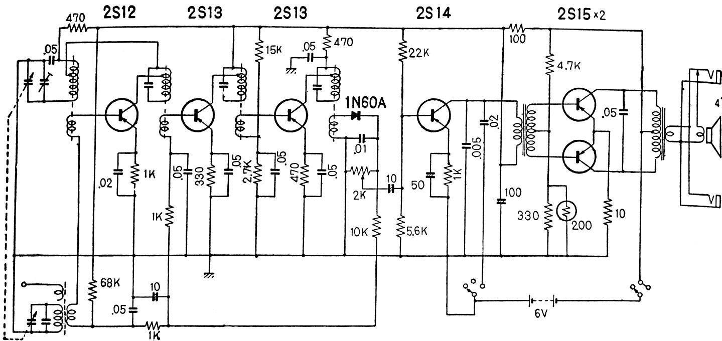
TOSHIBA 6TR-92.
