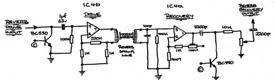
Vox Venue Dual 100 Pre-Amp
