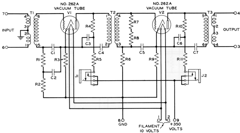
Fig. 2—Schematic Diagram of No. 69A Amplifier
