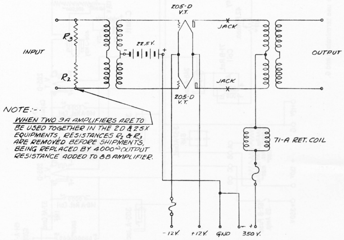
SCHEMATIC OF MODIFIED 9A. AMPLIFIER FOR OPERATION ON A.C. FIL. CURRENT SUPPLIED FROM TA-7114 PANEL.
