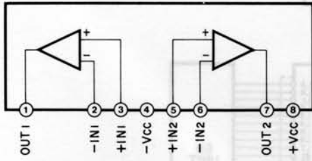
IC101, 111: M5218L (V) Dual Op-Amp
