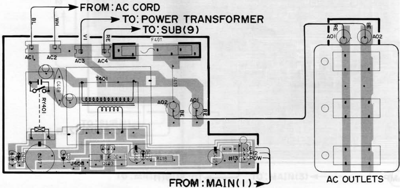
Sub Circuit Board (3)
