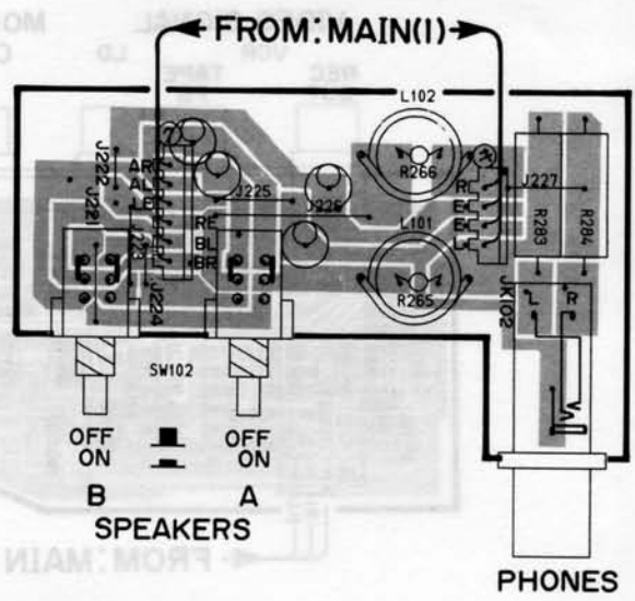
Main Circuit Board (4)
