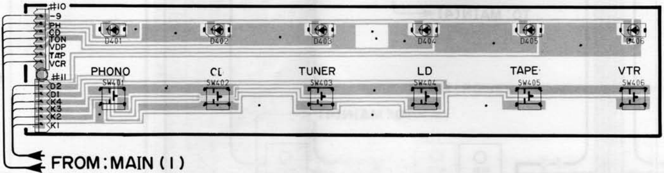
Sub Circuit Board (2)
