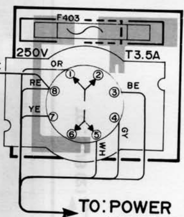
VOLTAGE SELECTOR
