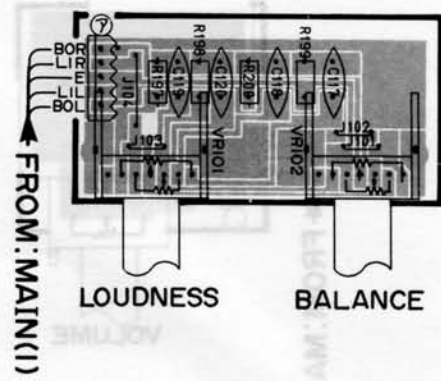
Main Circuit Board (2)
