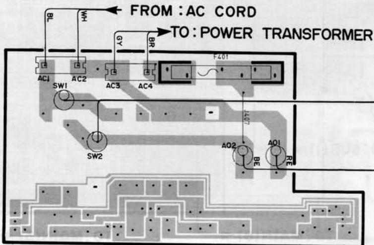
Sub Circuit Board (3)
