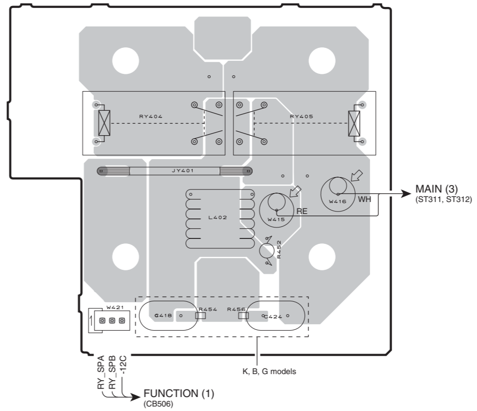
FRONT (16) (Side A)
