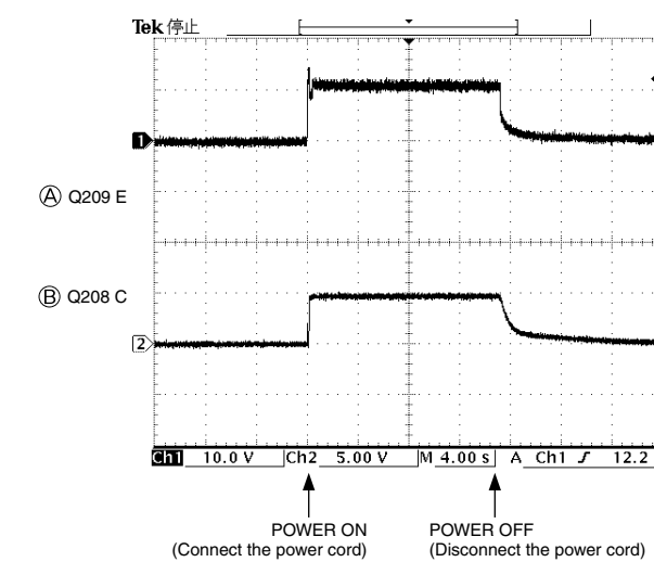
Point ④ emitter of Q209 and collector of Q208
