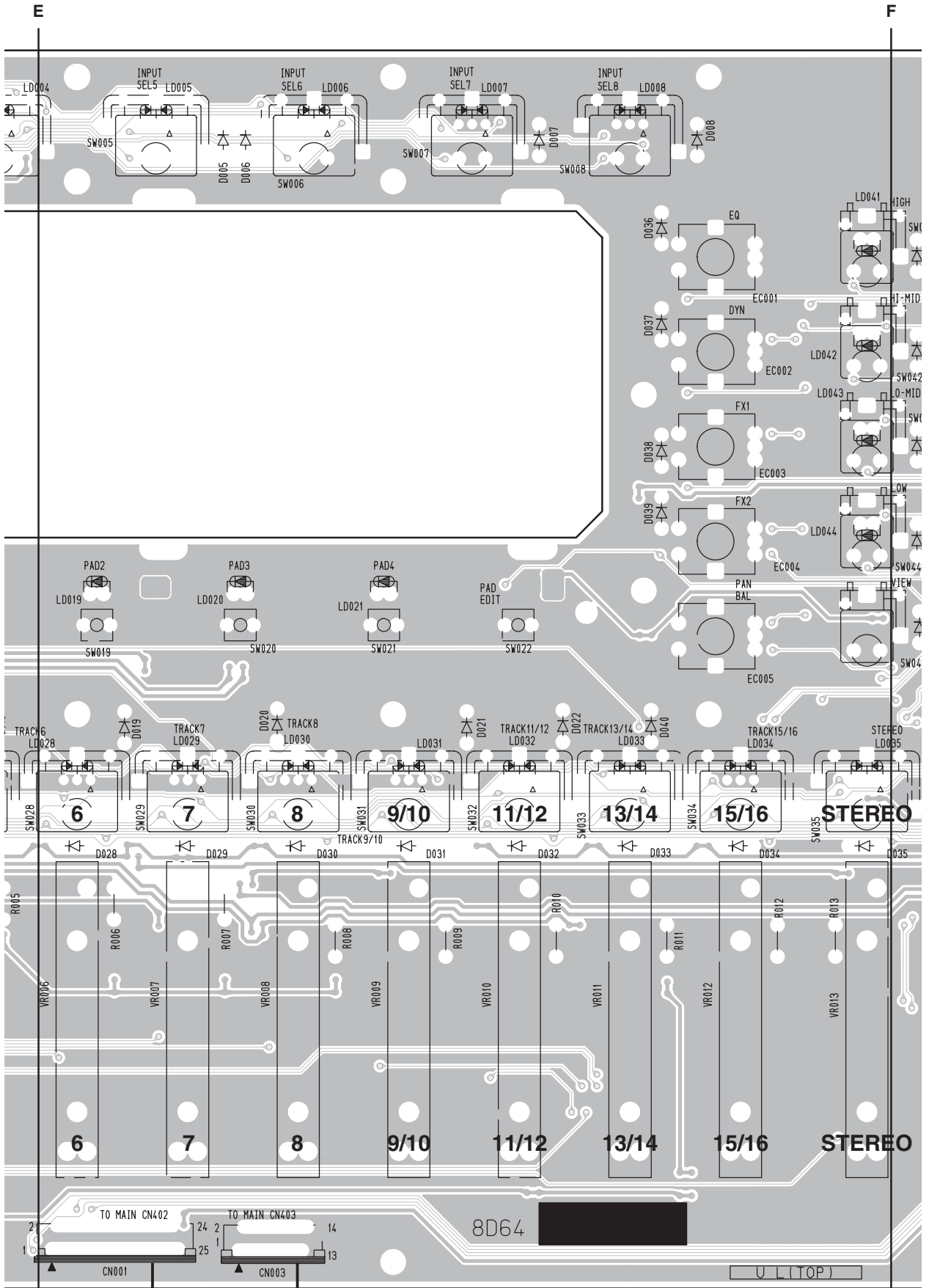
E' to MAIN-CN402 to MAIN-CN403 2NAP-WD39930 Component side (部品側) F'
