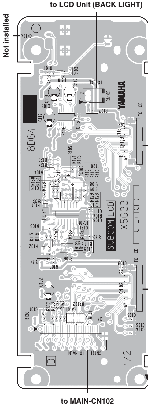
Component side (部品側)
