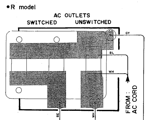
Sub Circuit Board (3)
