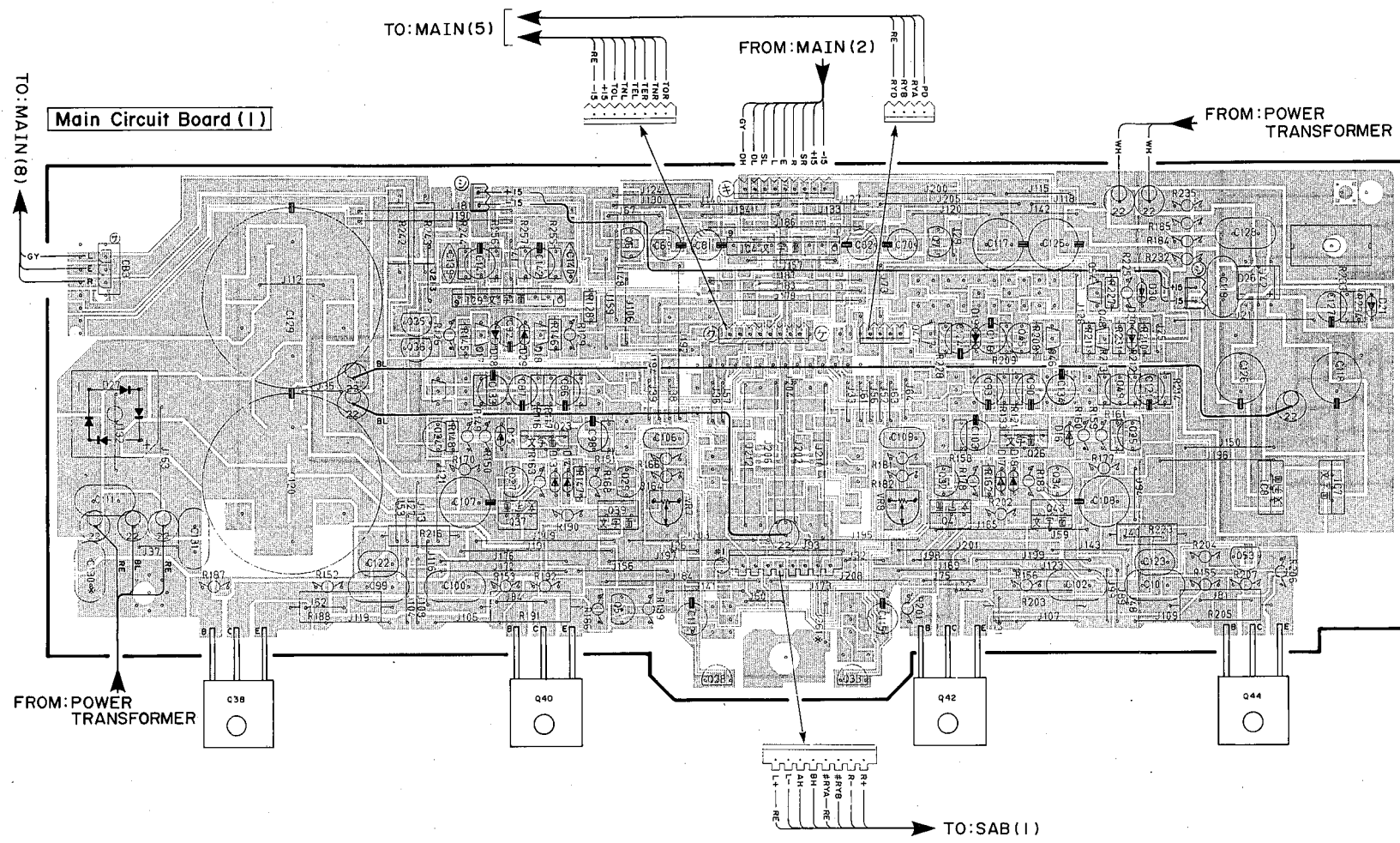
Main Circuit Board (1) (Chip Side)
