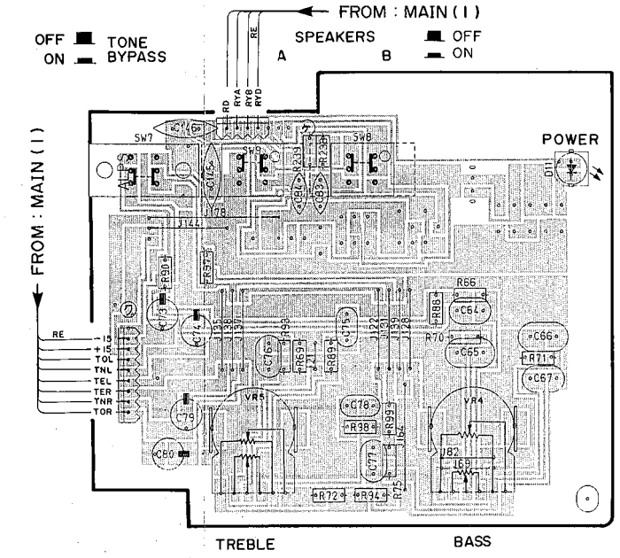
Main Circuit Board (5)
