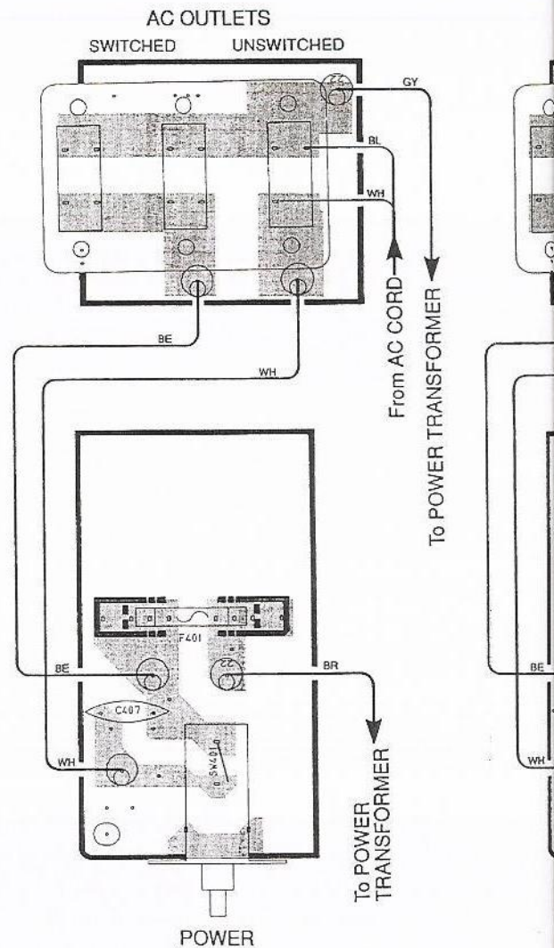
SUB CIRCUIT BOARD (2)
