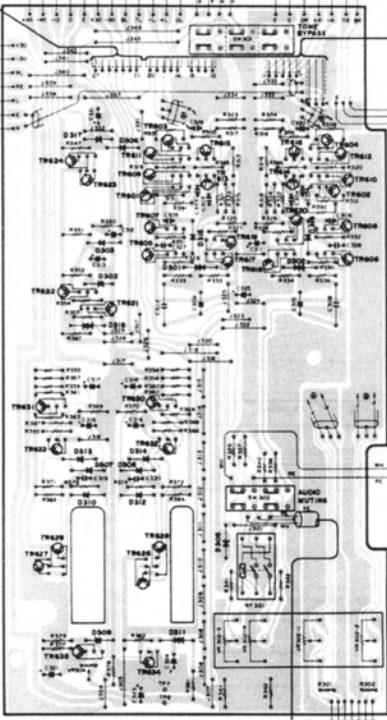
FLAT AMP C BOARD(2) NA07151-2 (U: NA07182-2)
