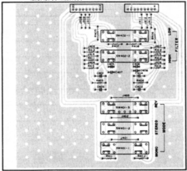
SWITCH C BOARD NA07157 (U: NA07189)
