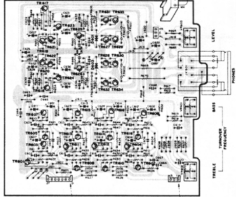
HEAD PHONE C BOARD NA07155 (U: NA07186)
