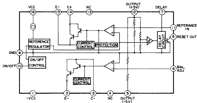
IC13 : M5290P Constant-Voltage Tracking Supply with Reset
