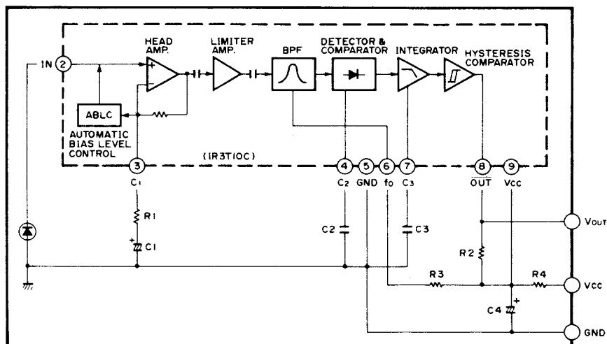
U401 : GPIU501X Remote Control Receiver Unit
