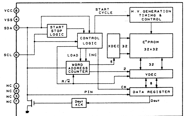
IC7 : X24C01P Electrically Erasable PROM
