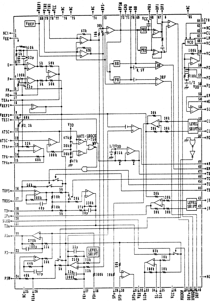
IC3 : BA10358, \mu PC358C or LM358N IC4 : MC1458N or BA1521B IC13, 14 : NJM2068D-D IC10, 11 : NJM5532D-D IC12 : BA1521B Dual OP-Amp
