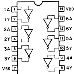
IC16 : PC74HCU04 Hex Inverter
