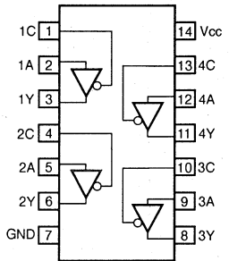
IC16 : HD74HC125AP Quad 3 State Bus Buffers
