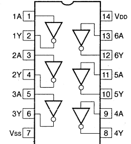
IC18 : TC74HCU04AP Hex Inverter
