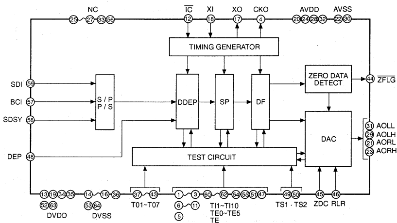
IC17 : YAC514 D/A Converter
