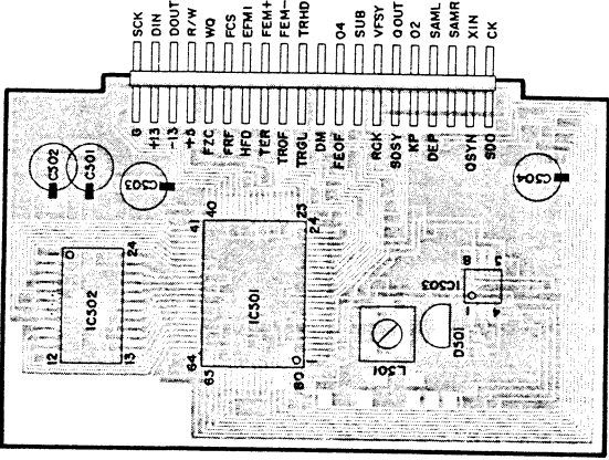
S/C Circuit Board ... Parts side
