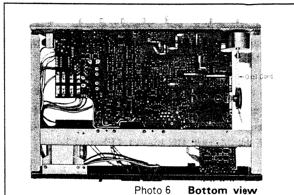
Photo 6 Bottom view
