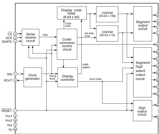
IC801: M66003-0131FP-R 18 digit 5 x 7 segment VFD controller/driver
