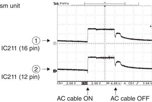
POINT (B) ① / Pin16, ② / Pin12 of IC211
