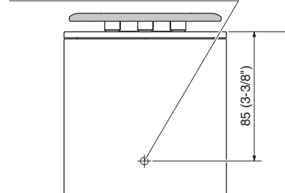
NS-BP110 Bottom view
