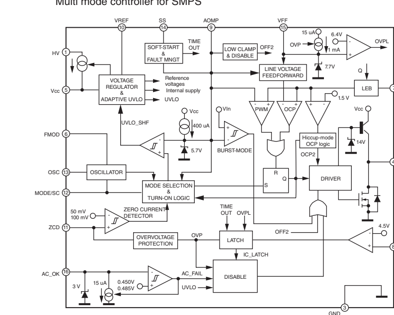
IC1: L6566BTR Multi mode controller for SMPS
