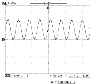
POINT (A) XL202 (Pin 15 of IC211)
