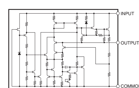
IC13: NJM7812FA Voltage regulator
