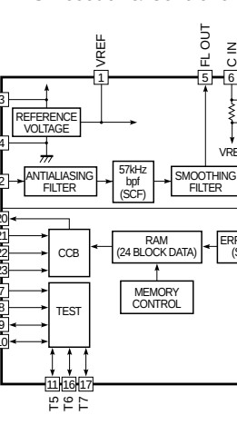
IC109 : LC72722 RDS Decoder & Controller
