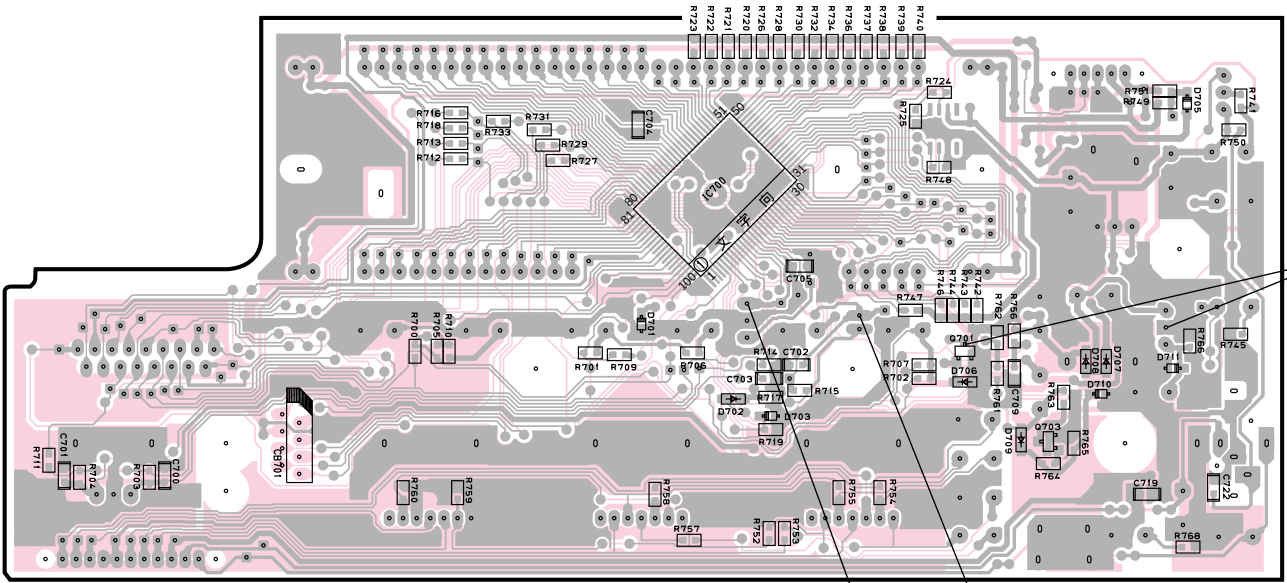
OPERATION P. C. B. (Surface Mount Device View)
