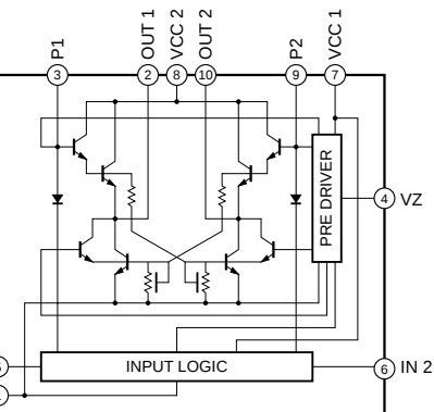
IC211 : LB1641 Motor Driver
