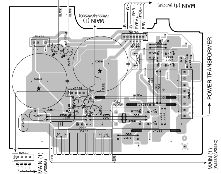
MAIN (2) P.C.B. (Side A)
