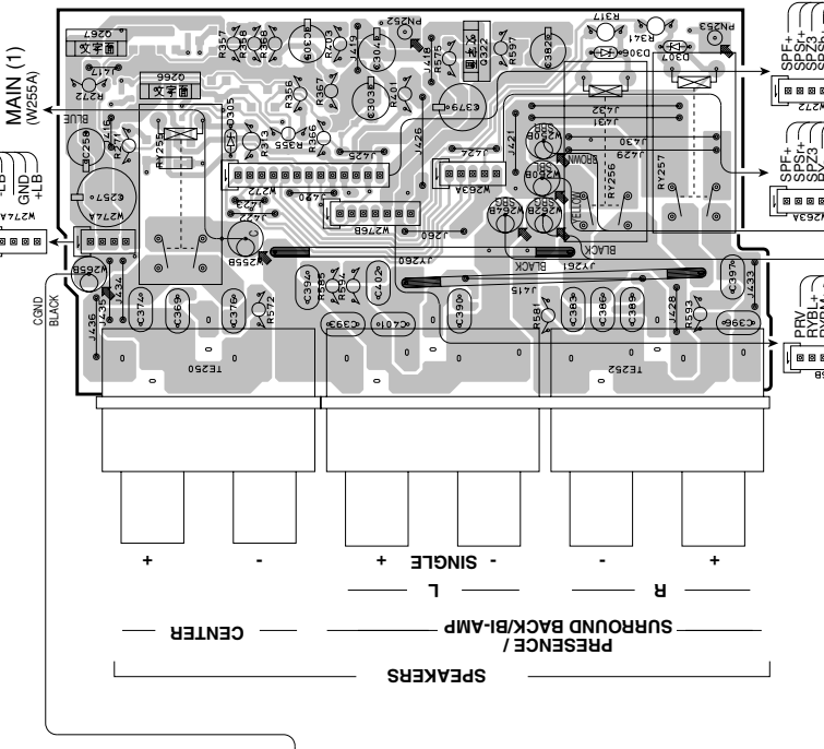
MAIN (4) P.C.B. (Side A)
