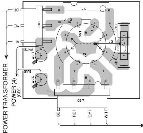
POWER (2) P.C.B. (Side A) R, L models
