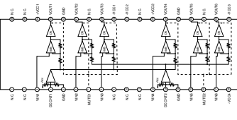
IC218: LA75930-TLME Analog data operational amplifier
