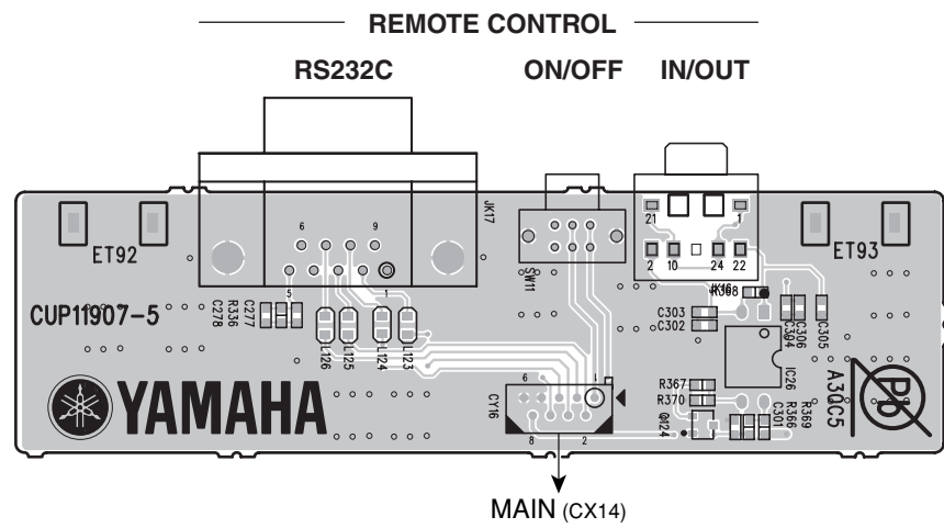
VIDEO (5) P.C.B. (Top view)
