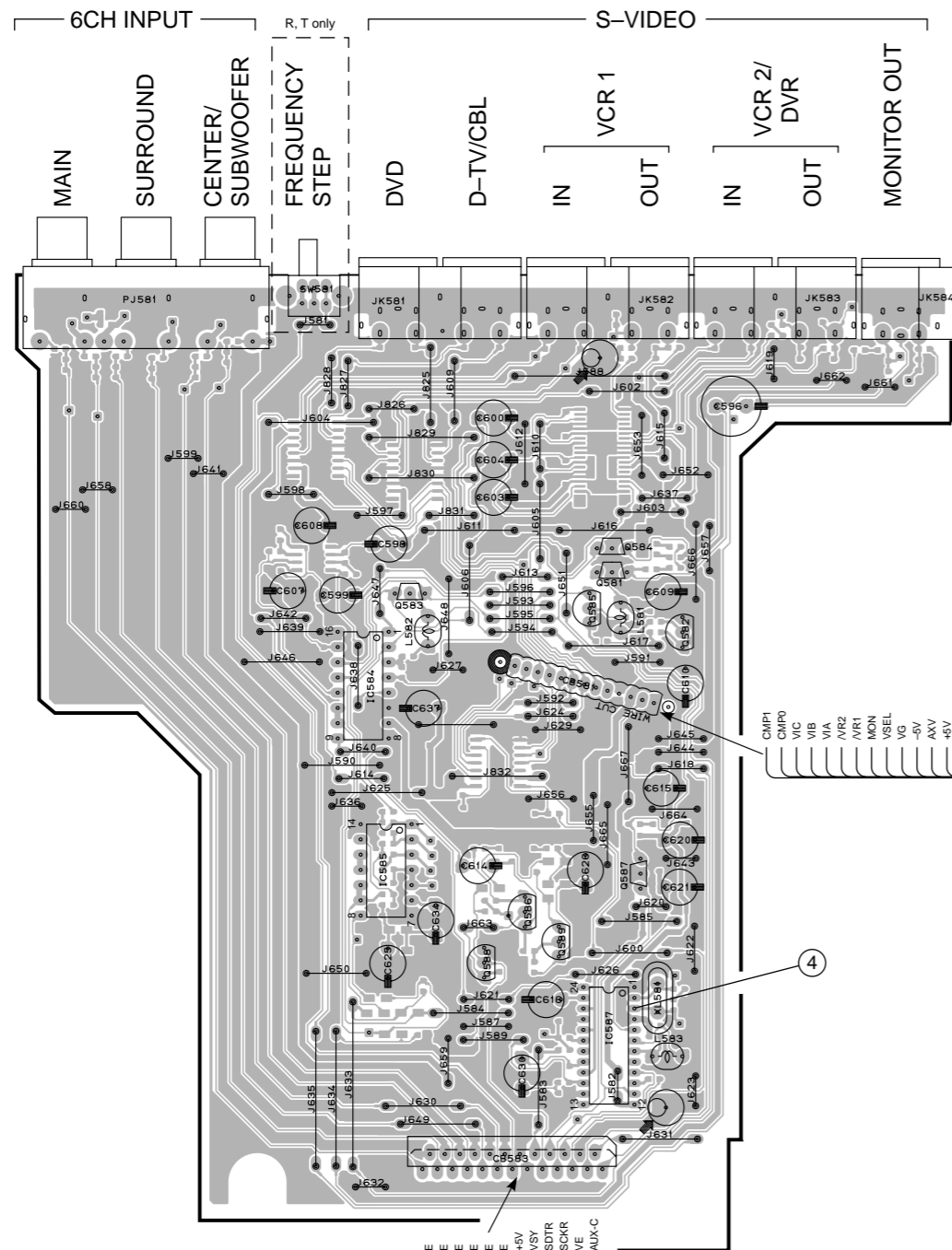
OPERATION ( 2 ) P. C. B. (Lead Type Device)
