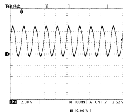
Point ③ Pin 12 of IC571
