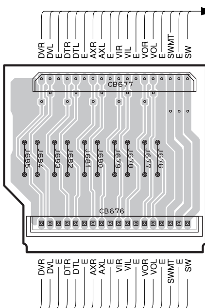
FUNCTION (6) P. C. B. (Side B) Lead Free Solder Used
