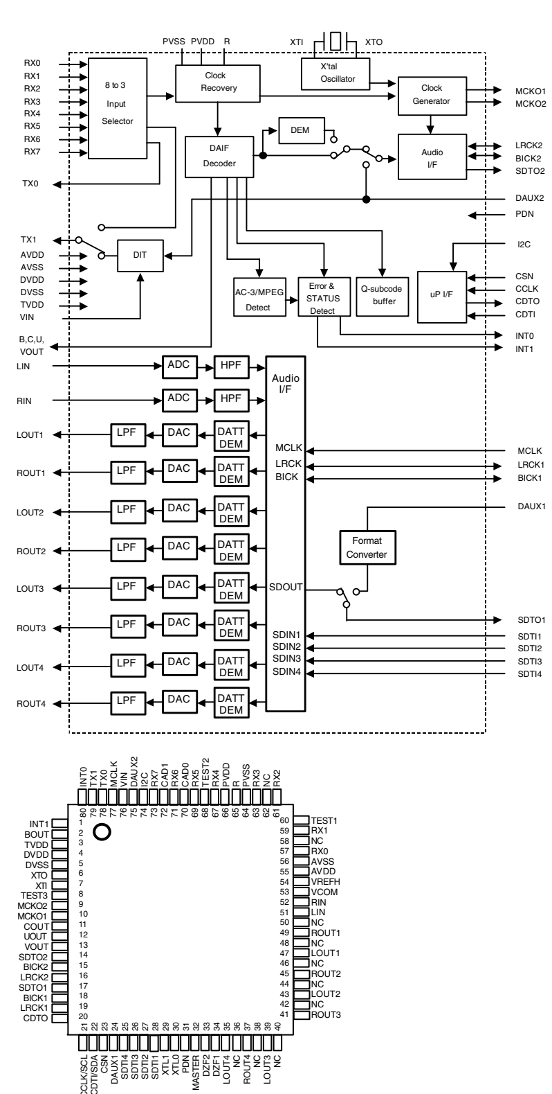
IC301: AK4588VQ 2/8-channel audio CODEC with DIR
