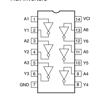
IC305: SN74LV04APWR Hex inverters
