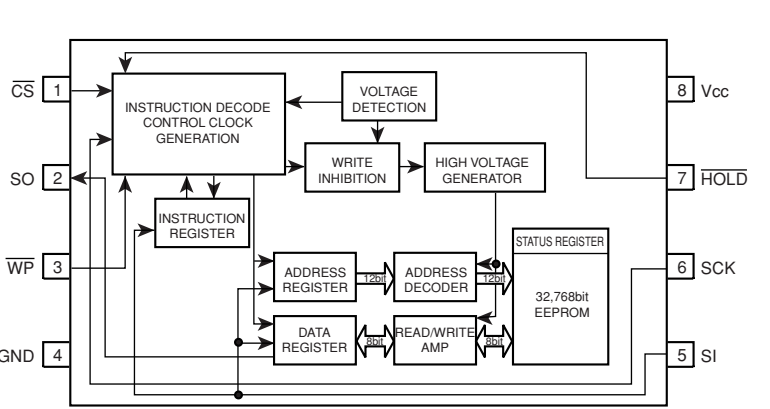
IC102: BR25L320F-W EEPROM SPI BUS 32 k-bit (4,096 x 8-bit) EEPROM
