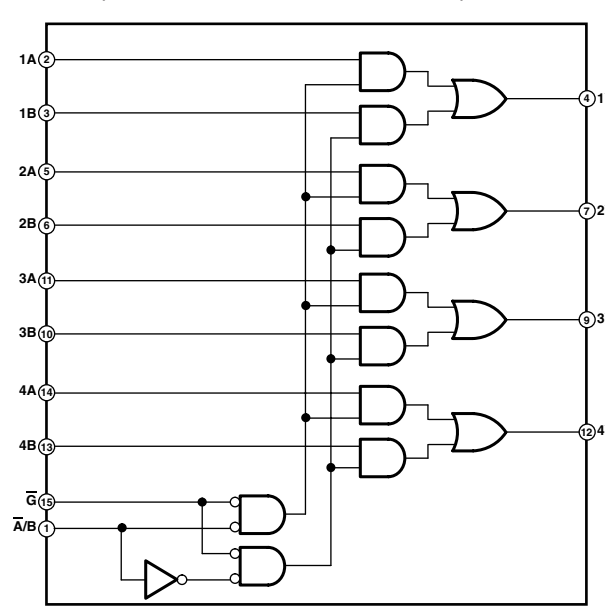
IC302: SN74LV157APWR Quaduple 2-line to 1-line data selectors/multiplexers
