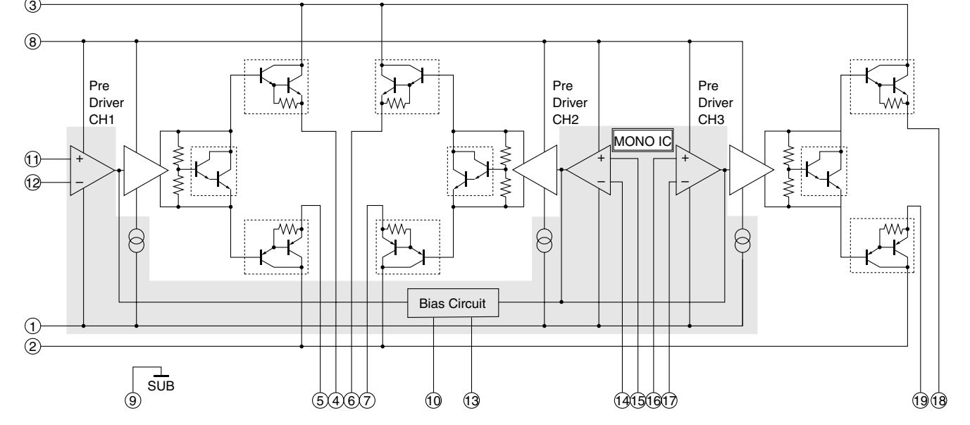
IC101: STK433-330-E 3-channel AF power amplifier, stand-by circuit built-in
