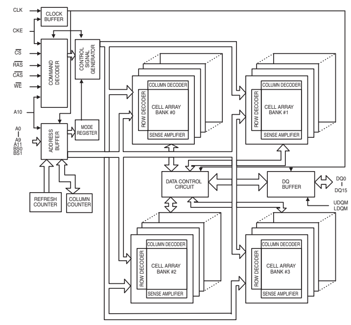
IC202: W9864G6EH-7 1 M x 4 Banks x 16-bit SDRAM
