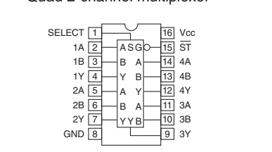
IC62: TC74VHC157FT
