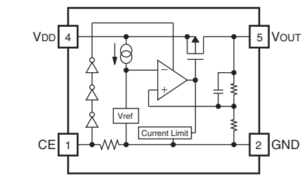
IC73: R1172H181B-T1-F Voltage regulator
