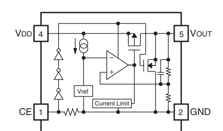
IC74: R1172H31D-T1-F Voltage regulator
