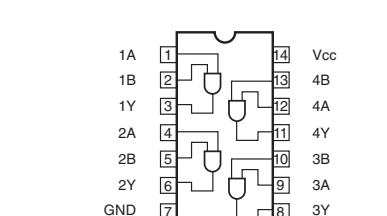
IC67: TC74VHC08AFT
