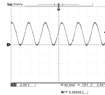
POINT F XL301 (Pin 3 of IC309)
