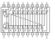
IC171B SN7ALV185APWR 33V ABT octal bus transceiver with 3-state output
