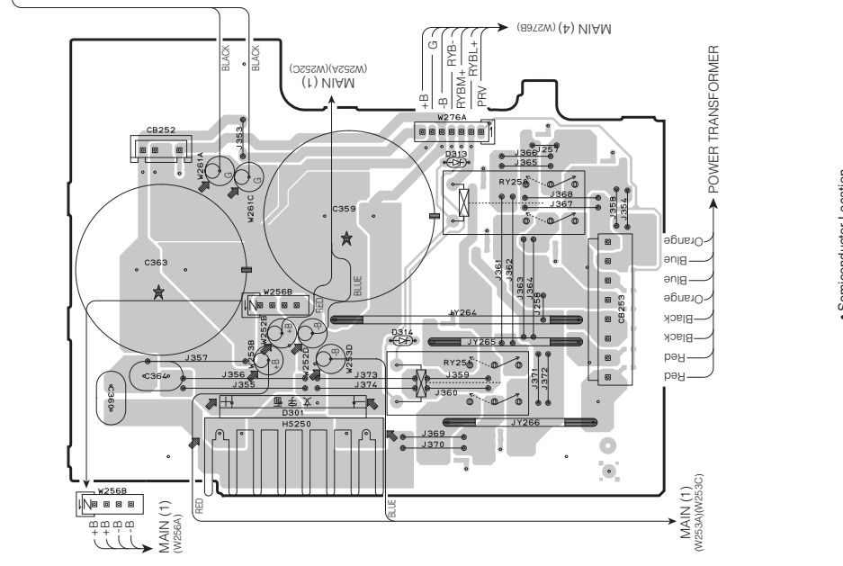
MAIN (2) P.C.B. (Side A)
