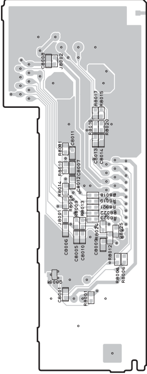
OPERATION (2) P.C.B. (Side B)
