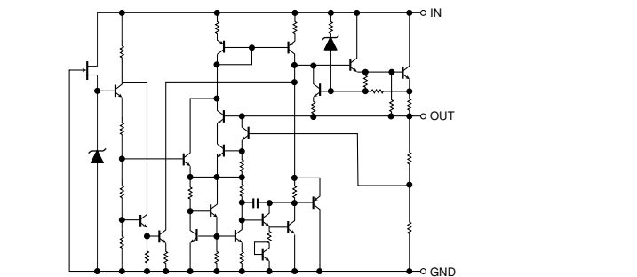
IC10, 12: NJM78M05FA 3-terminal positive voltage regulator
