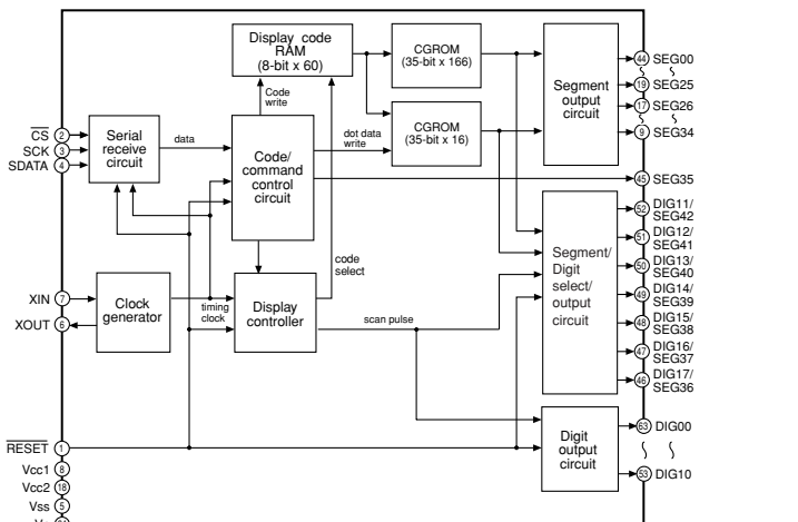
IC901: M66003-0131FP-R 18 digit 5 x 7 segment VFD controller/driver
