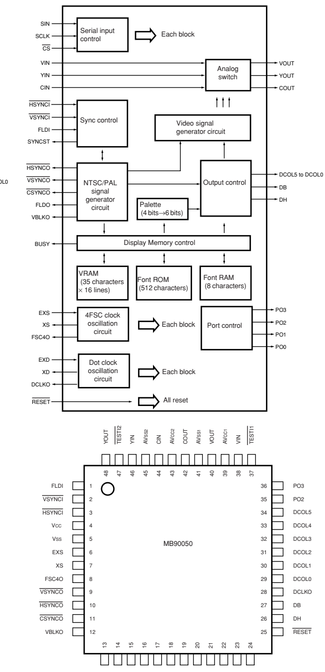
IC8: MB90050PF-G-119-E1 OSD controller
