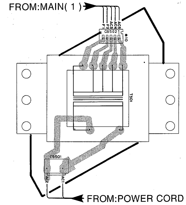
● Except R model P.C.B. MAIN ( 5 )
