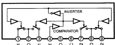
IC1 : μPC1330HA 2ch Head Selector Switch
