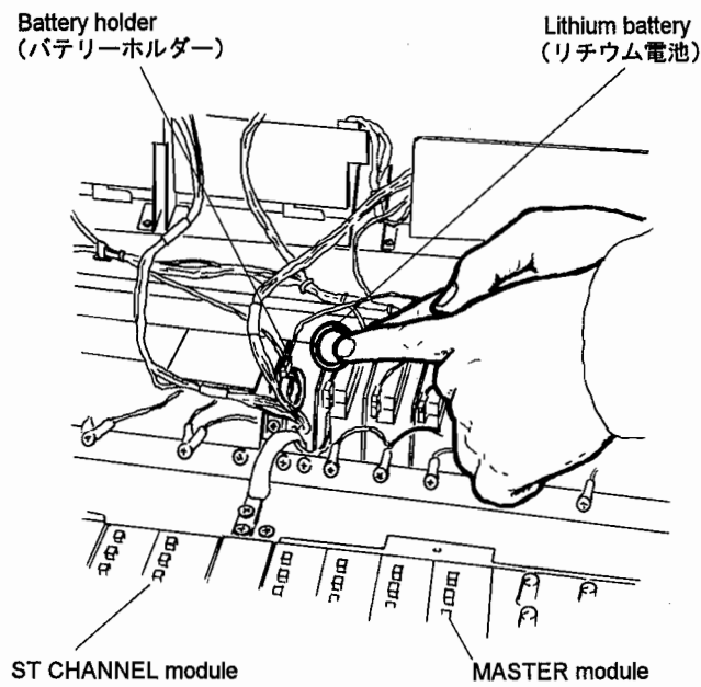
(Fig. 12) Lithium Battery
