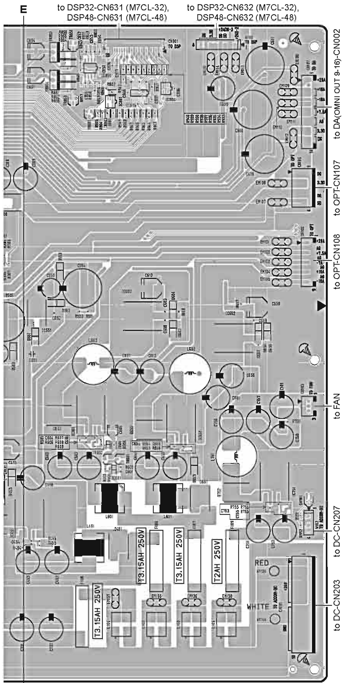
Component side (部品側)
